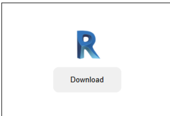
Figure 10: Download button.
