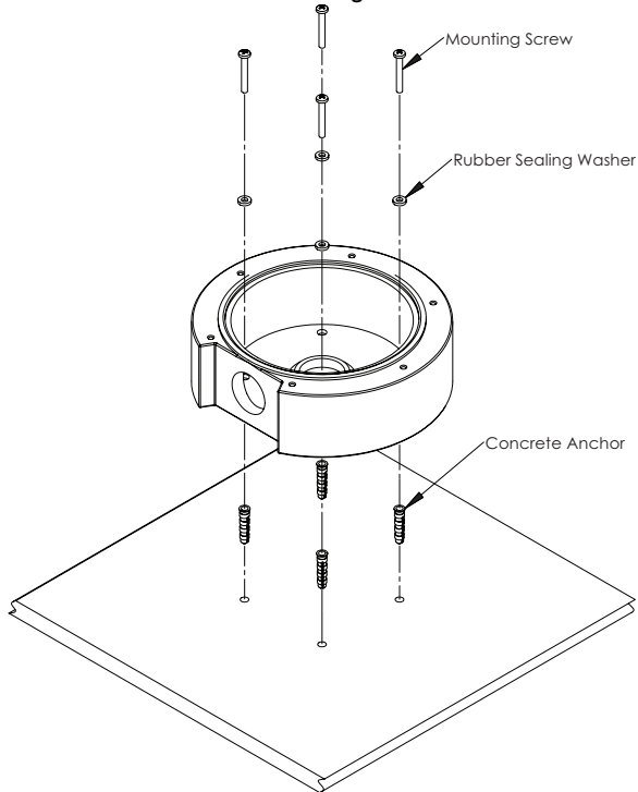
Figure: Indoor/Outdoor Mounting Base Installation
