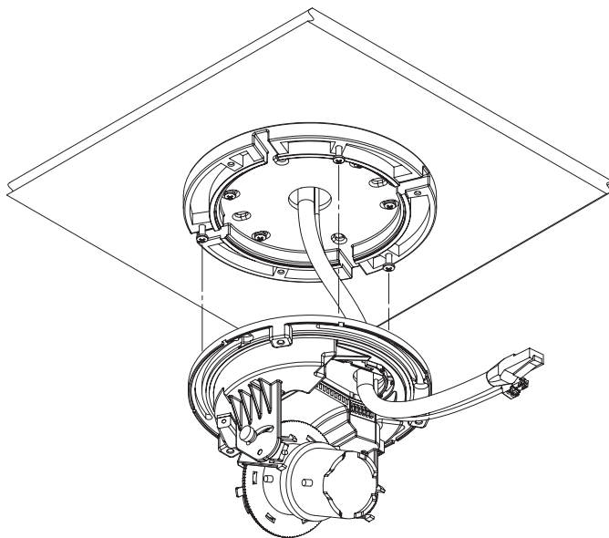
Figure: Dome Camera Installation
