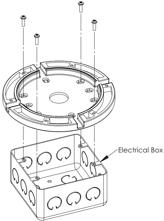
Figure: Indoor Electrical Box Mounting Plate Installation
